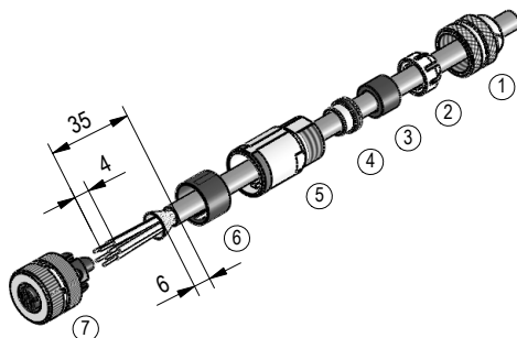
Fig. 2: Straight mating connector M12
