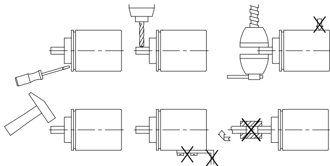
Fig. 1: Mounting instructions
