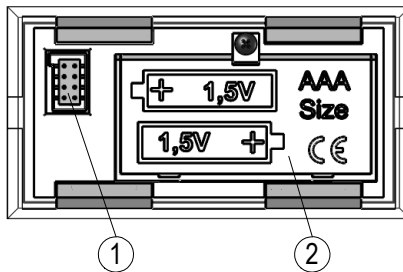
Fig. 3: Connection
