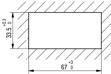
Fig. 1: Panel mounting
