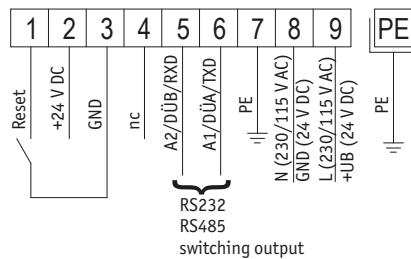
Fig. 3: Connection diagram
