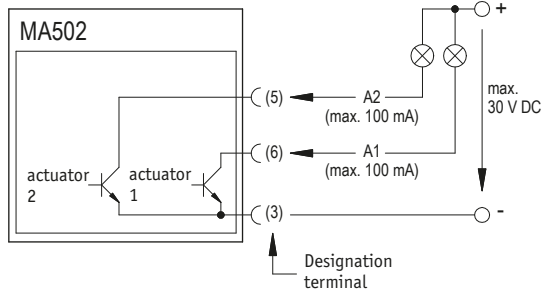
Fig. 6: Connection diagram switching outputs
