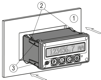
Fig. 1: Installation
