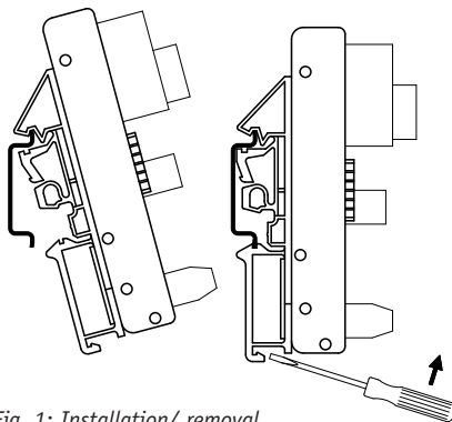
Fig. 1: Installation/ removal
