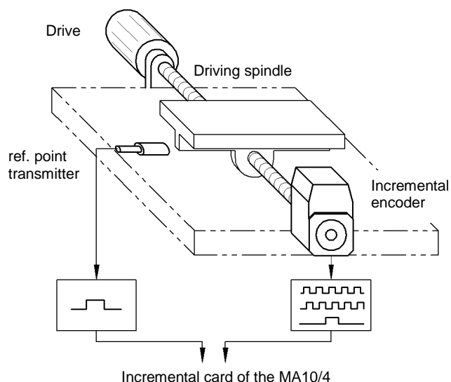
Fig. 3: Referencing setup
